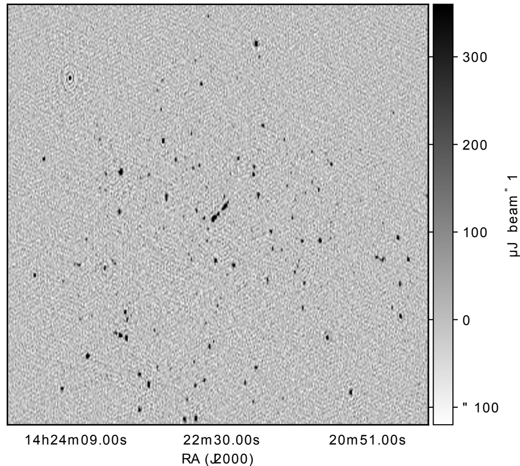
200425057 beam 11 DDC
