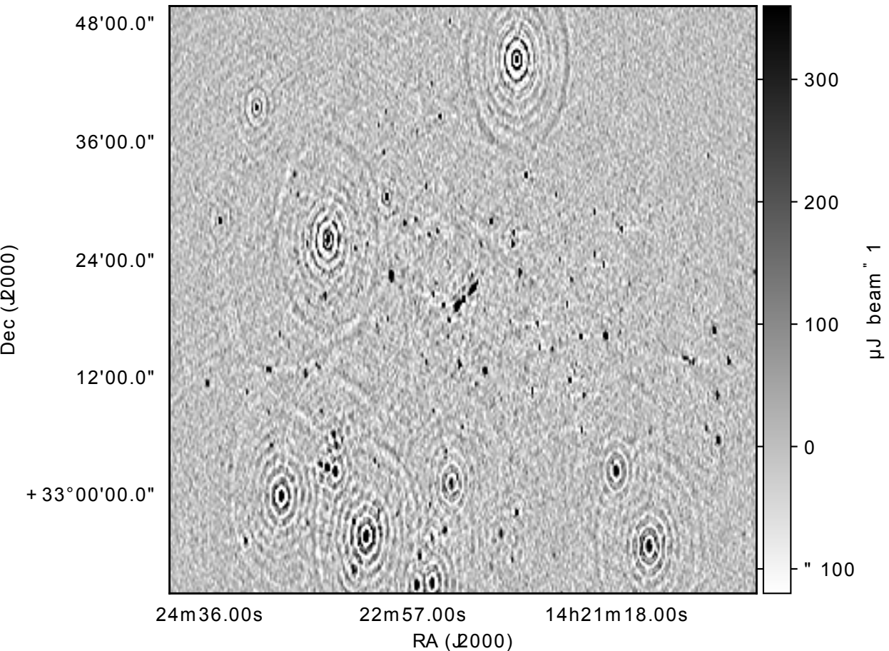
200425057 beam 11 Apercal
